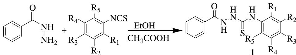
Scheme-1.1: Synthesis of Thiosemicarbazide derivatives.
